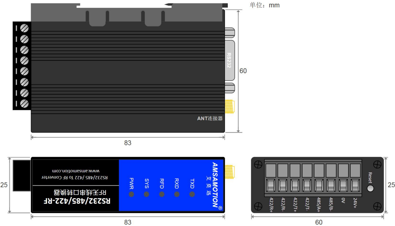
Figura 3.1 Diagrama dimensional de RS232/485/422-RF
